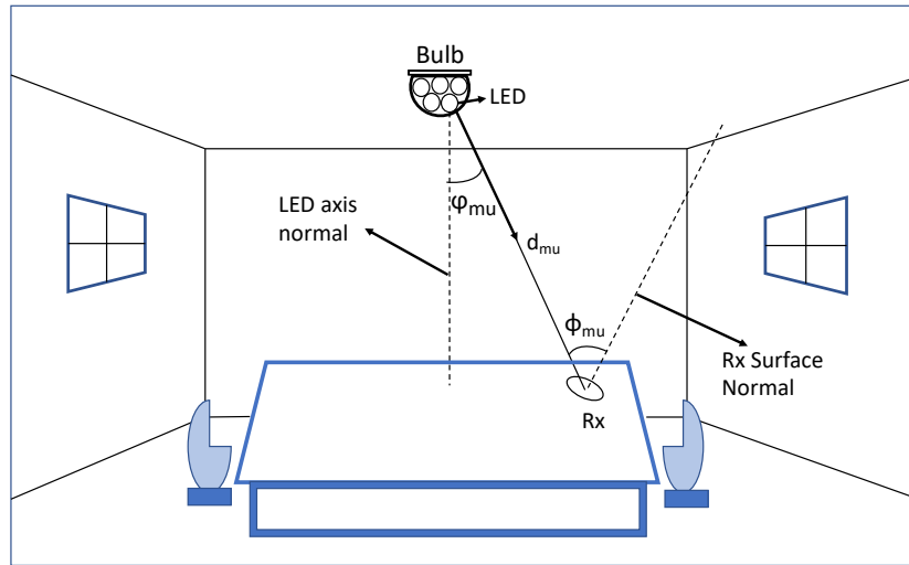
Figure 4.1: Transmitters and receivers in a VLC channel model
