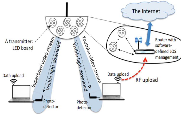
Figure 3.1: Design of a multi-element VLC architecture [5]
